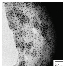
TEM image of dried magnetic biosol stabilized by readily available coal humic acids
